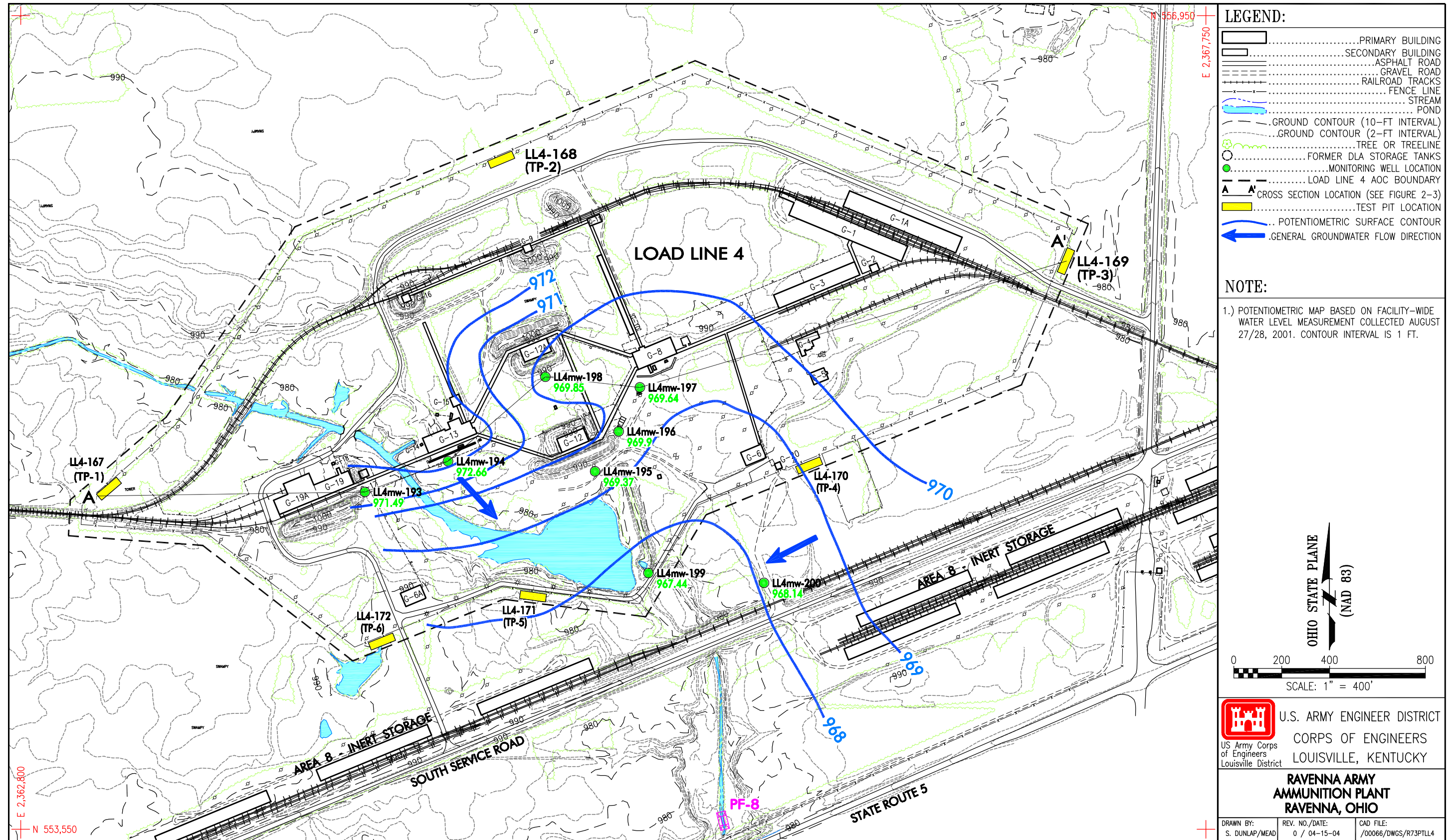
Figure 2-5. Potentiometric Groundwater Surface at Load Line 4, August 2001
