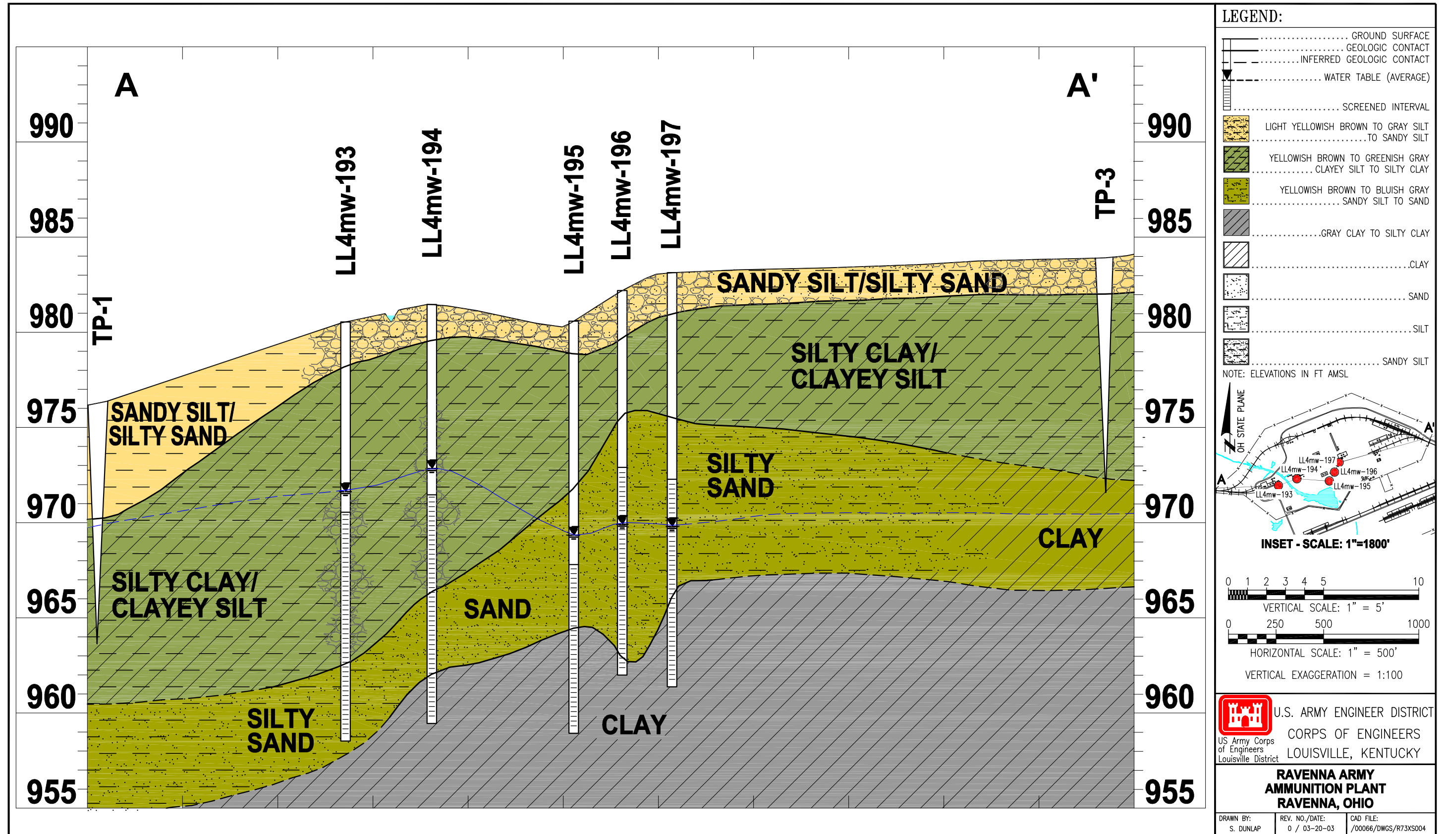
Figure 2-3. Generalized Geologic Cross Section at Load Line 4
