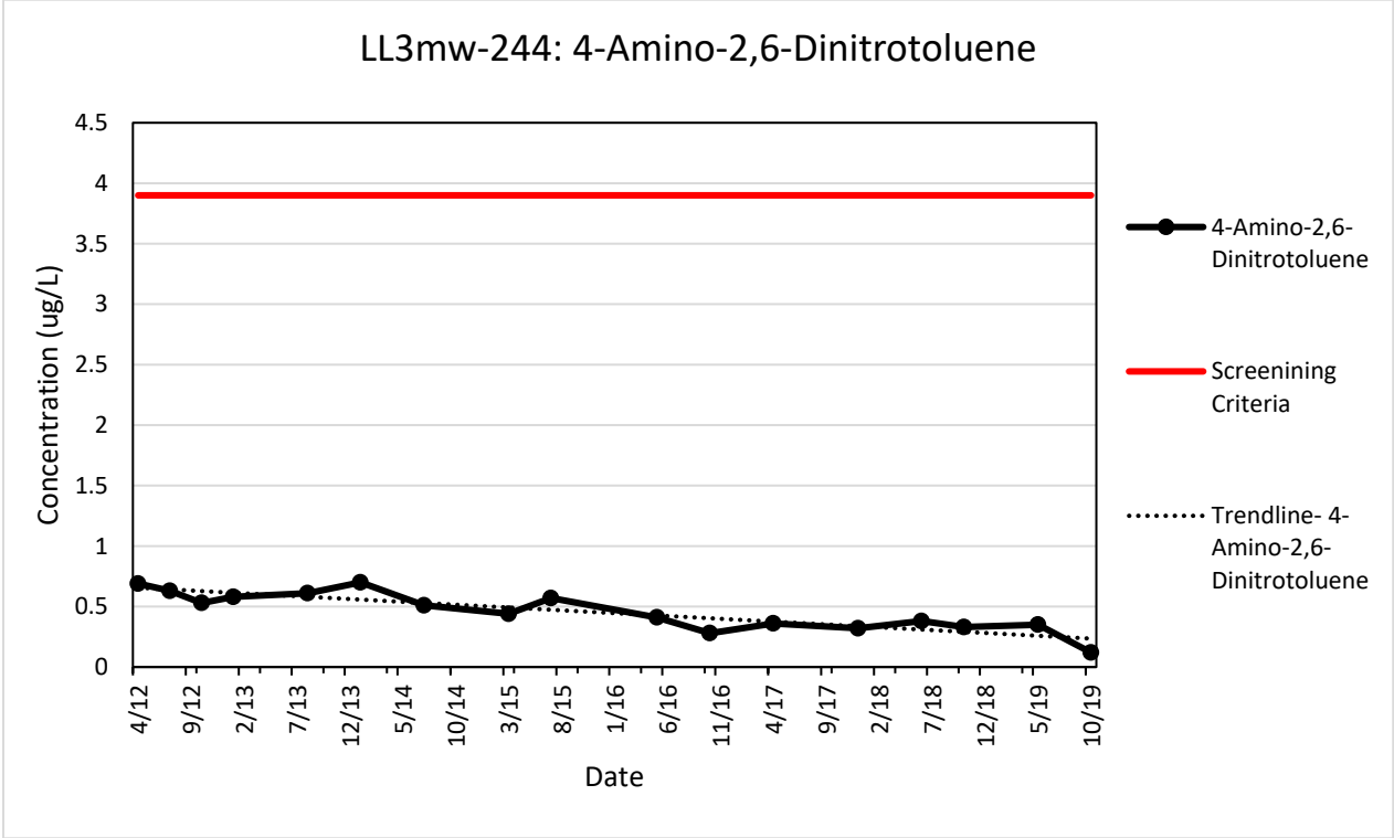
Figure G-36. LL3mw-244 Trendline for 4-Amino-2,6-Dinitrotoluene
