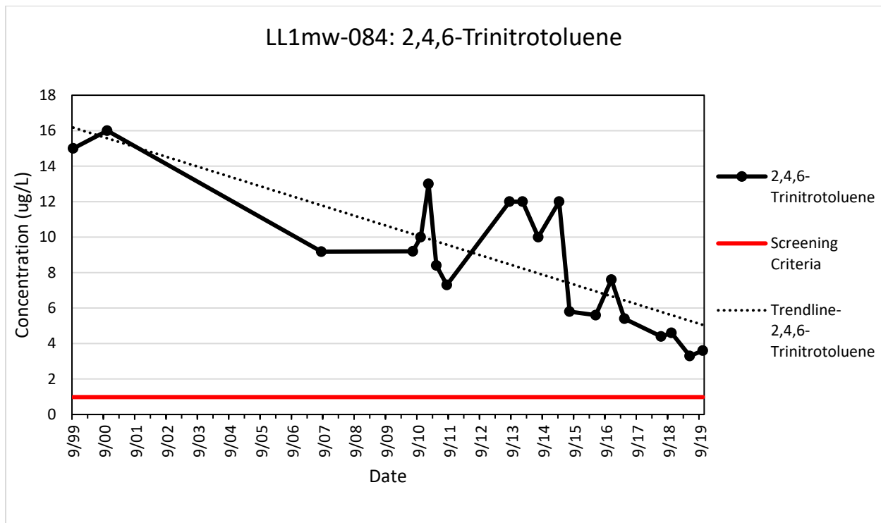
Figure G-18. LL1mw-084 Trendline for 2,4,6-Trinitrotoluene
