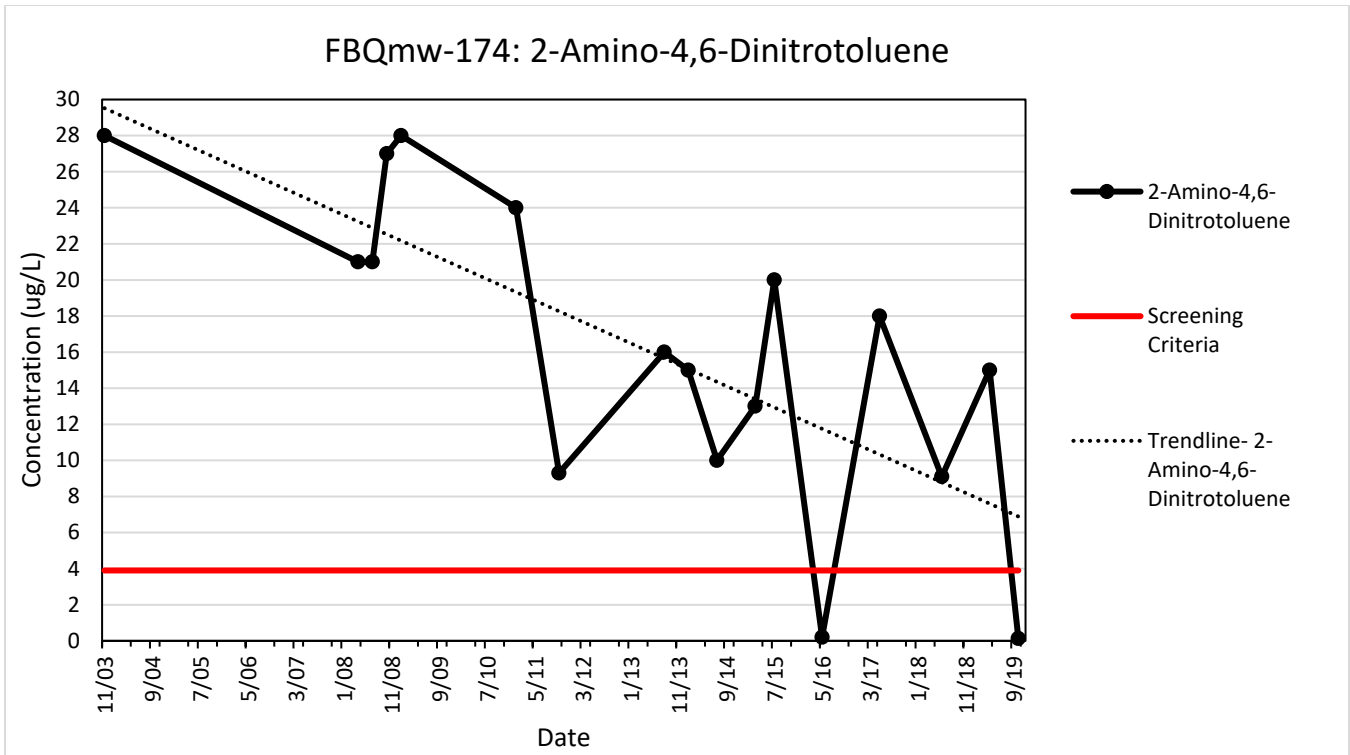
Figure G-3. FBQmw-174 Trendline for 2-Amino-4,6-Dinitrotoluene
