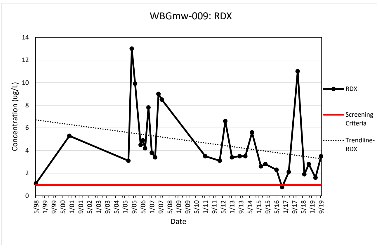
Figure G-40. WBGmw-009 Trendline for RDX
