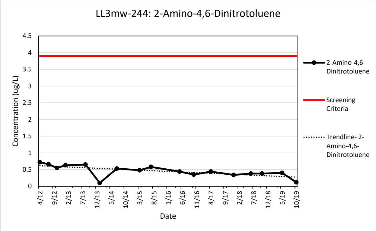
Figure G-35. LL3mw-244 Trendline for 2-Amino-4,6-Dinitrotoluene
