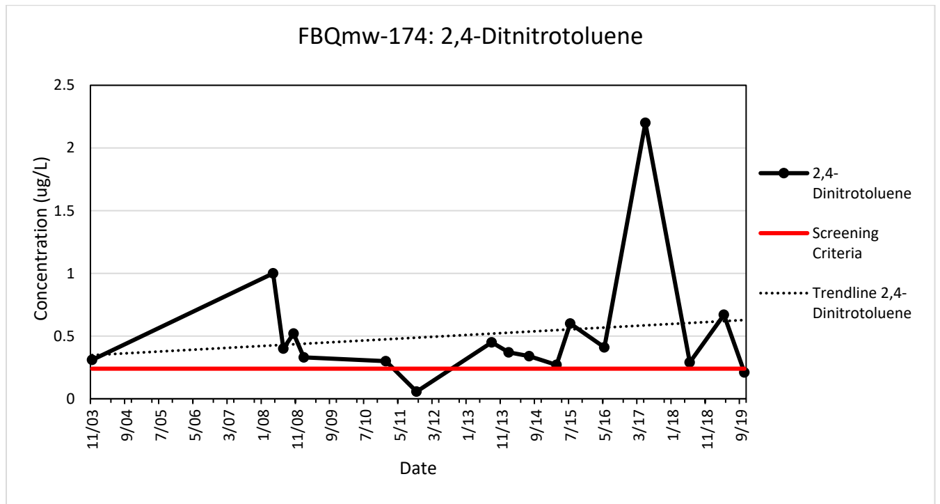
Figure G-2. FBQmw-174 Trendline for 2,4-Dinitrotoluene
