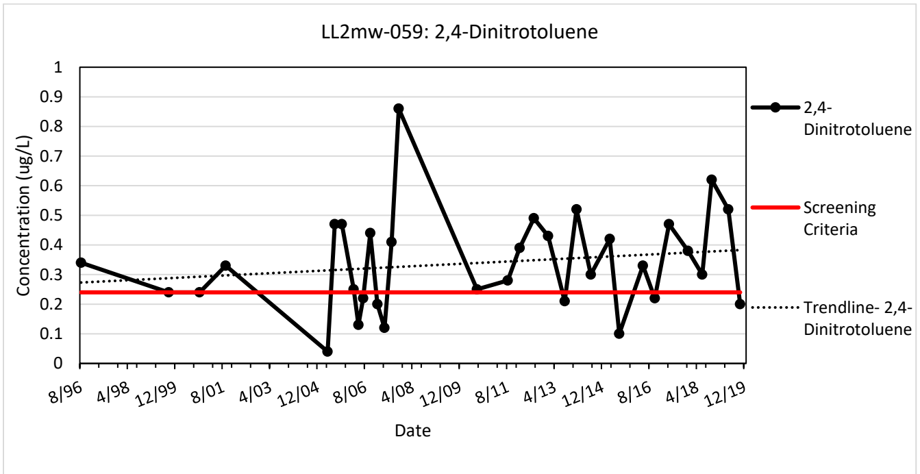
Figure G-23. LL2mw-59 Trendline for 2,4-Dinitrotoluene
