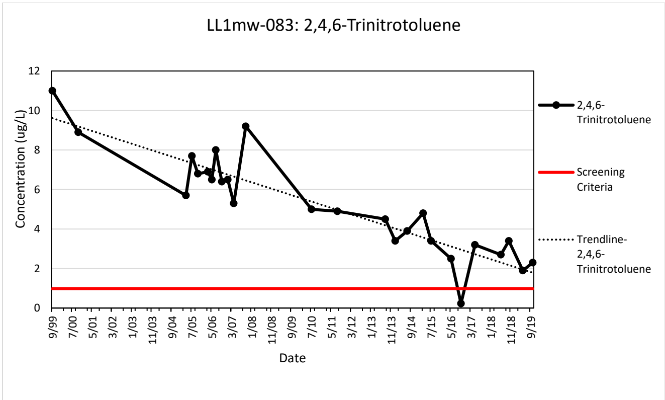
Figure G-13. LL1mw-083 Trendline for 2,4,6-Trinitrotoluene
