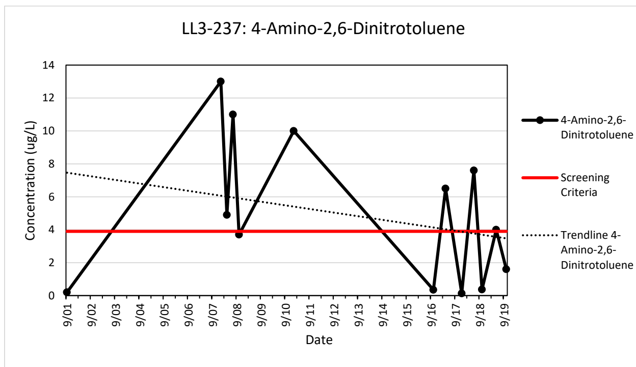
Figure G-34. LL3mw-237 Trendline for 4-Amino-2,6-Dinitrotoluene
