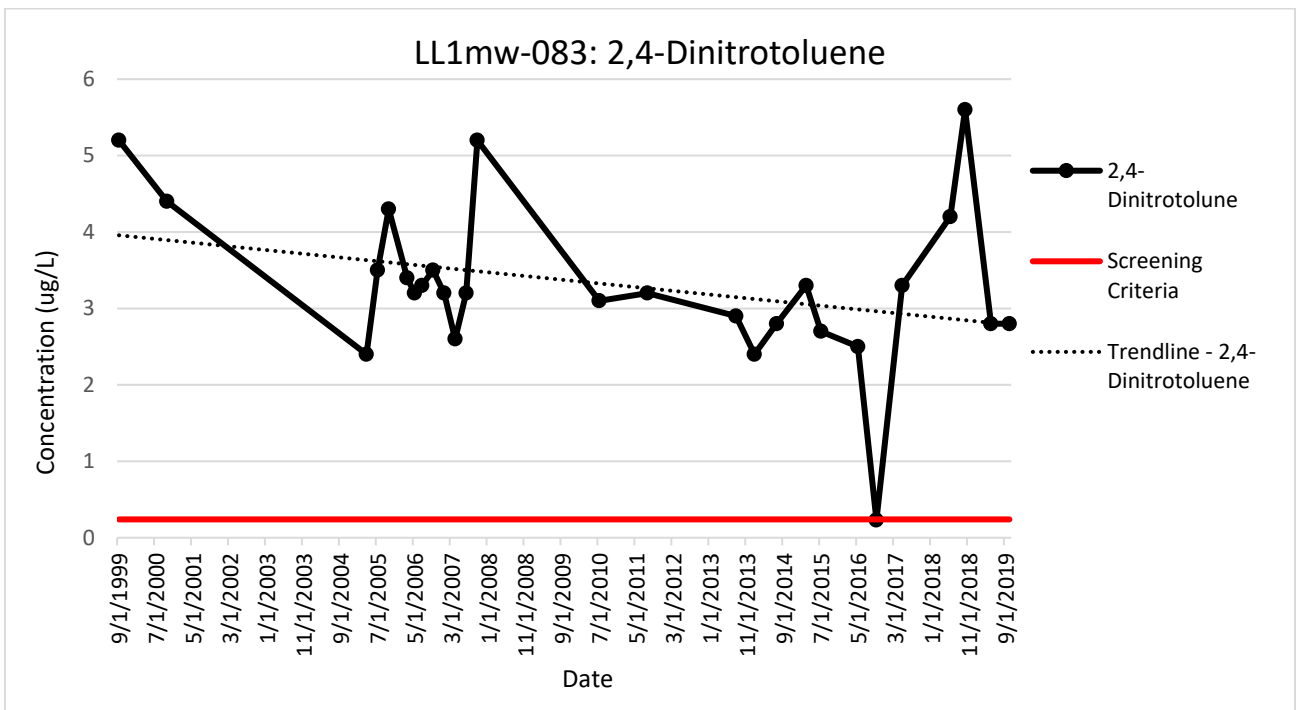
Figure G-14. LL1mw-083 Trendline for 2,4-Dinitrotoluene
