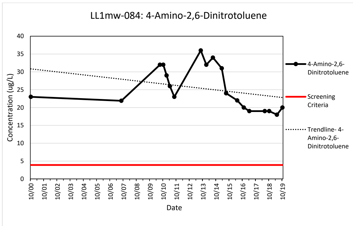
Figure G-20. LL1mw-084 Trendline for 4-Amino-2,6-Dinitrotoluene
