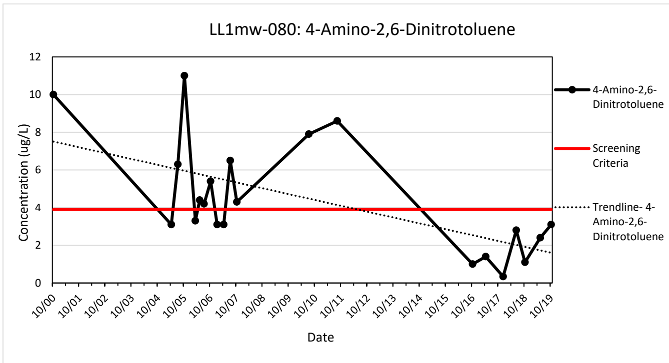
Figure G-8. LL1mw-080 Trendline for 4-Amino-2,6-Dinitrotoluene
