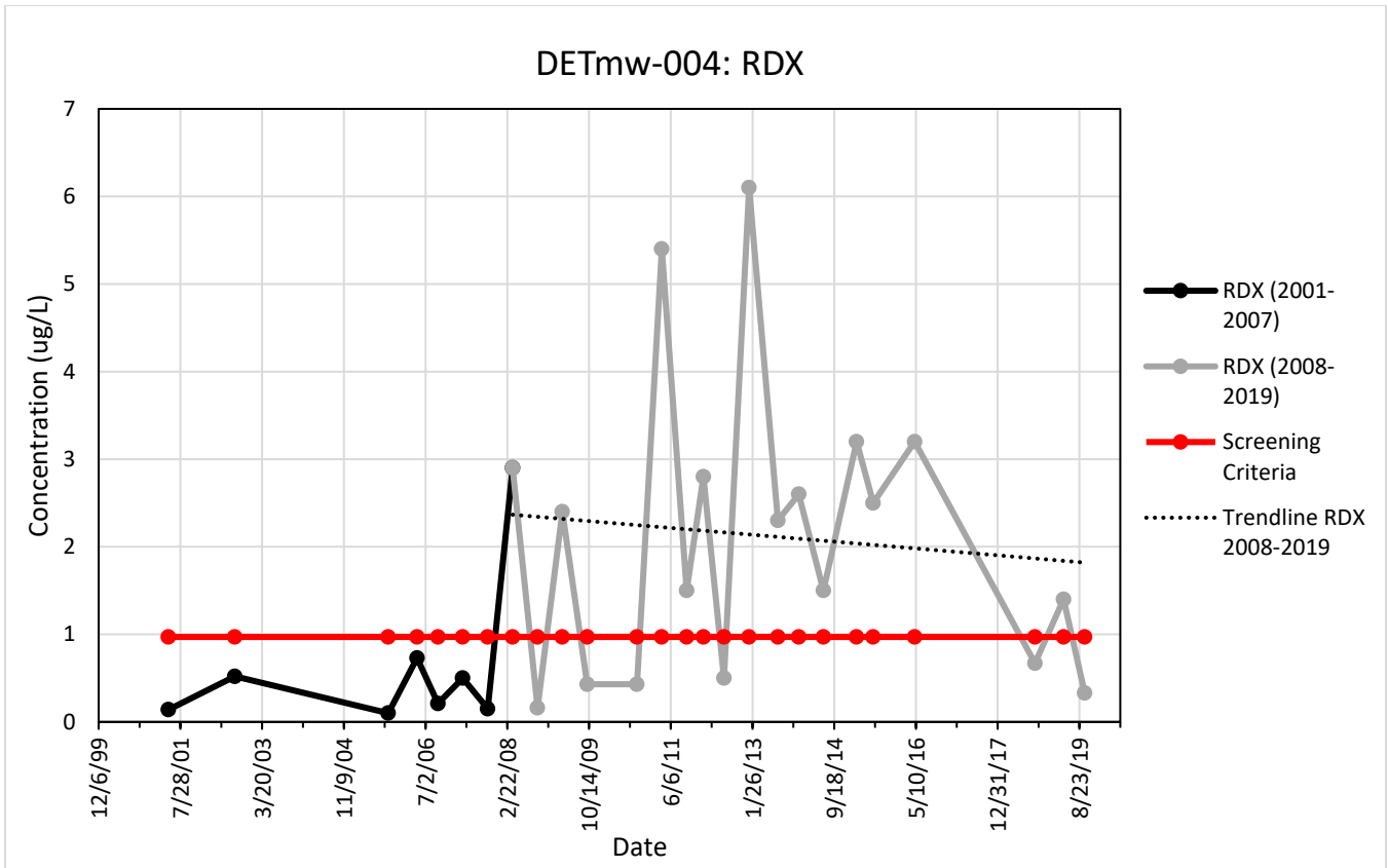
Figure G-1. DETmw-004 RDX Concentrations
