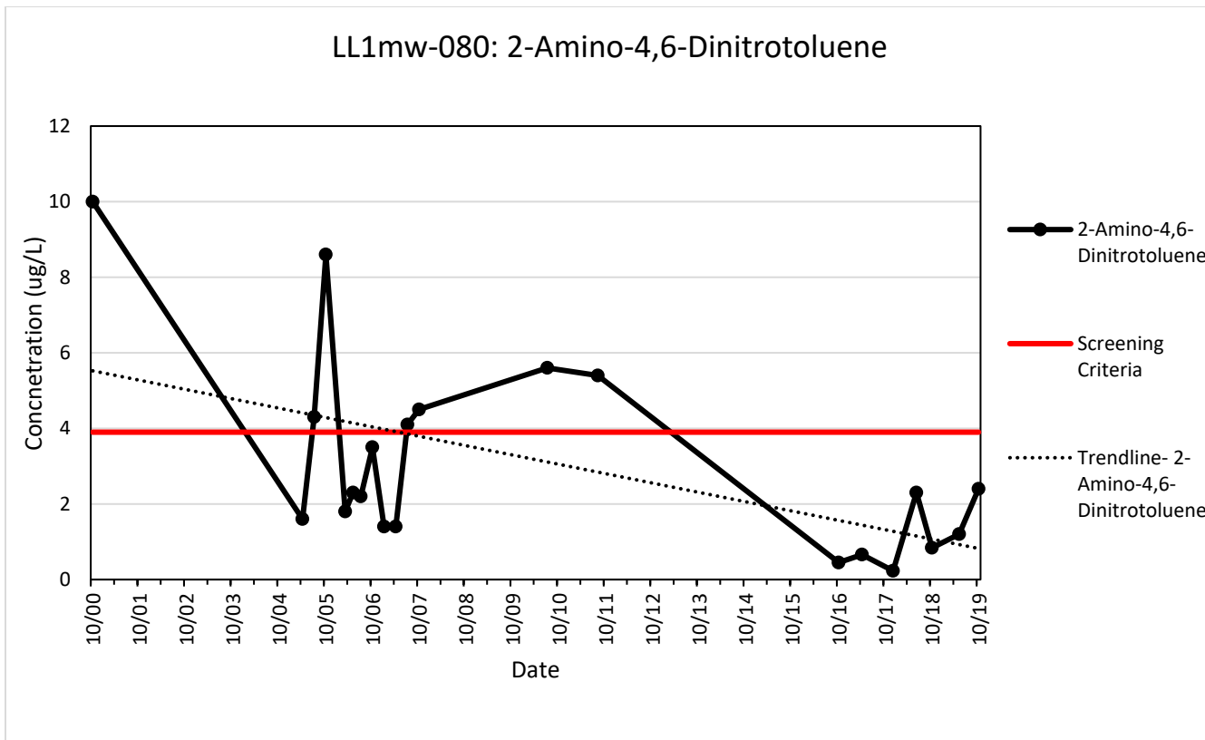
Figure G-7. LL1mw-080 Trendline for 2-Amino-4,6-Dinitrotoluene
