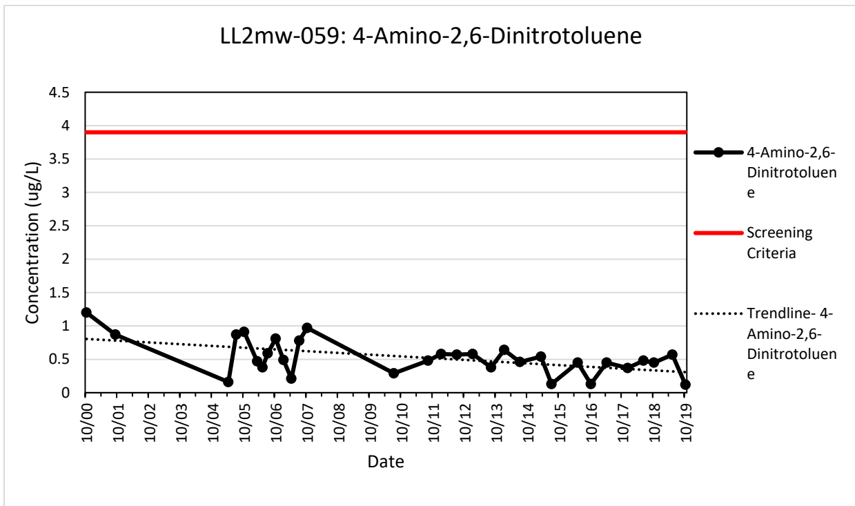
Figure G-24. LL2mw-059 Trendline for 4-Amino-2,6-Dinitrotoluene
