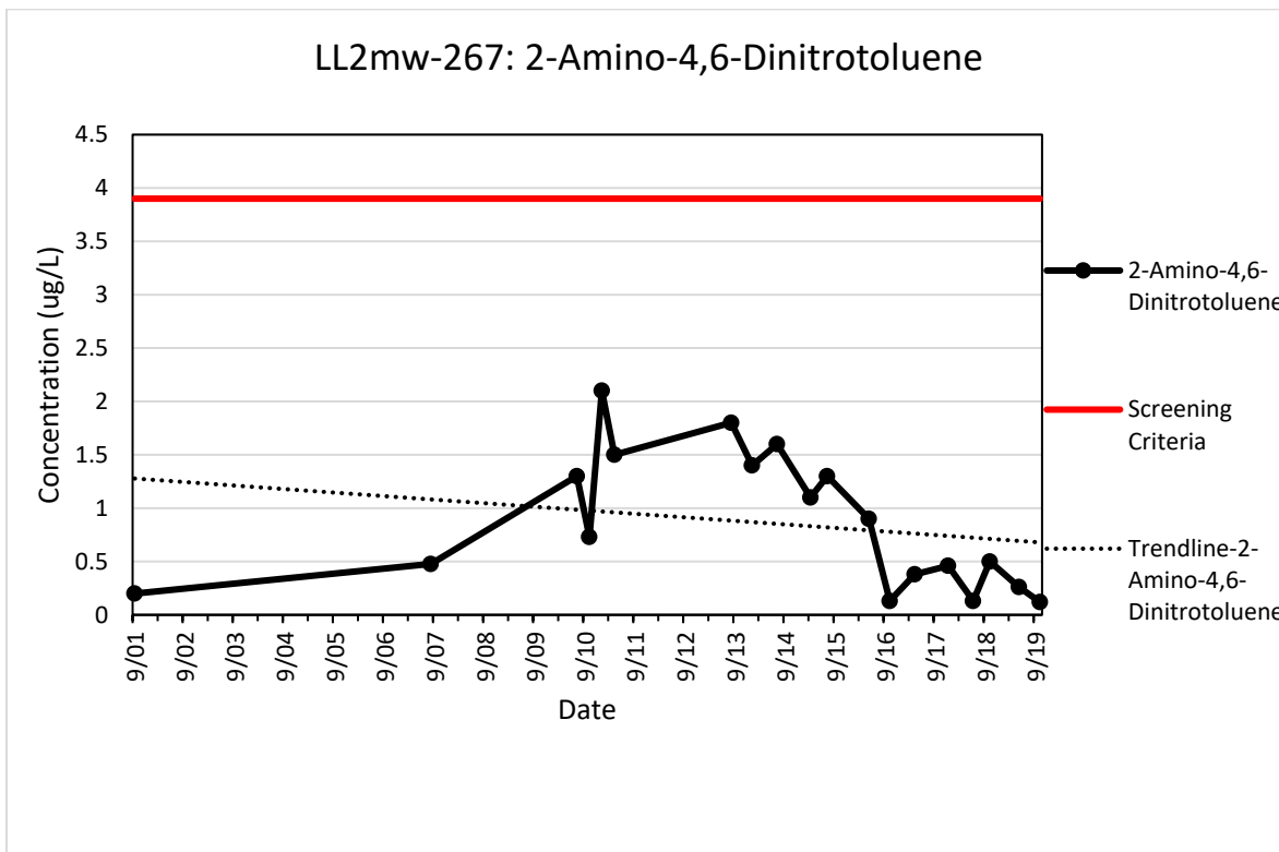
Figure G-30. LL2mw-067 Trendline for 2-Amino-4,6-Dinitrotoluene
